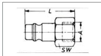
Racor macho
